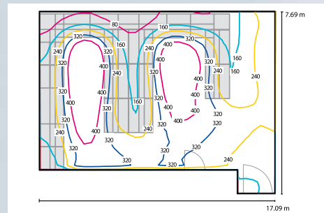
Light planning using ISO lines for indicating lighting intensities in Lux at any point of the room
