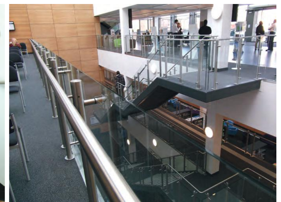
Left: Visually freestanding glass balustrade and applied handrail. Below Left: Nylon system with glass infill. Below Right: Stainless steel handrail and balustrading with glass infill.
