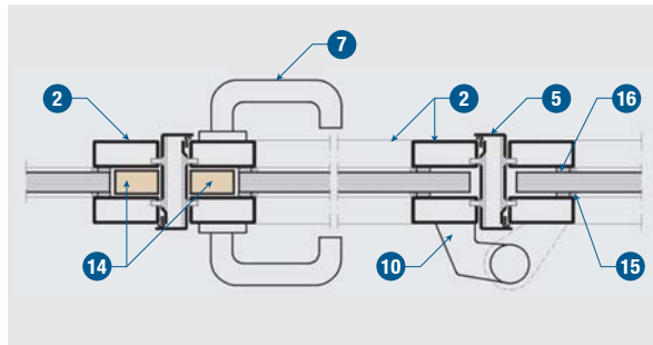
Detail 2 – Horizontal section (Section A-A).
