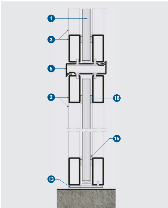
Detail 4 – Vertical section (Section C-C).
