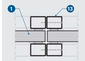
Detail 5 – Steel profile connection (Section B-B).
