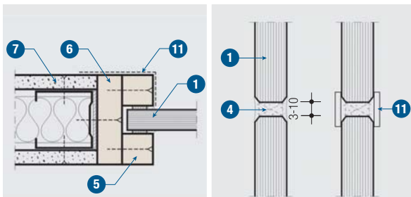
Detail 3 – Connection to lightweight partition (Section A-A).
