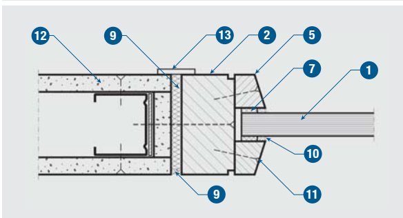
Detail 3 – Alternative connection to lightweight partition (Section A-A).
