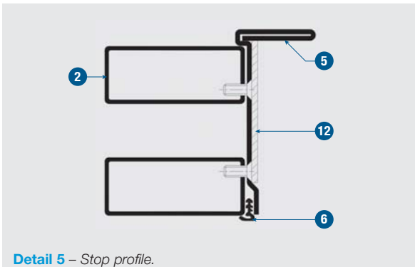
Detail 5 – Stop profile.
