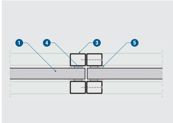
Detail 12 – Connecting steel profile.
