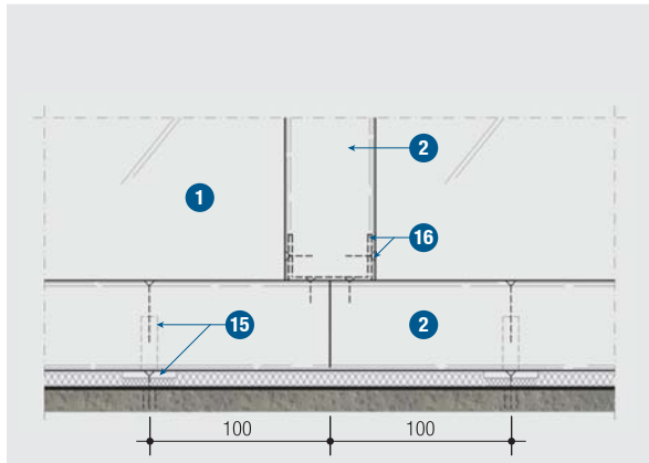
Detail 10 – Transom details.
