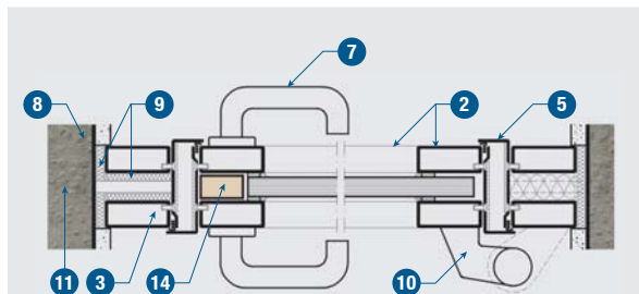
Detail 2 – Horizontal section (Section A-A).
