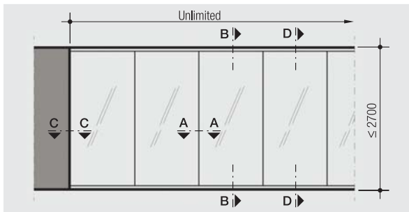
Detail 1 – Elevation (vertical & horizontal unframed joints).
