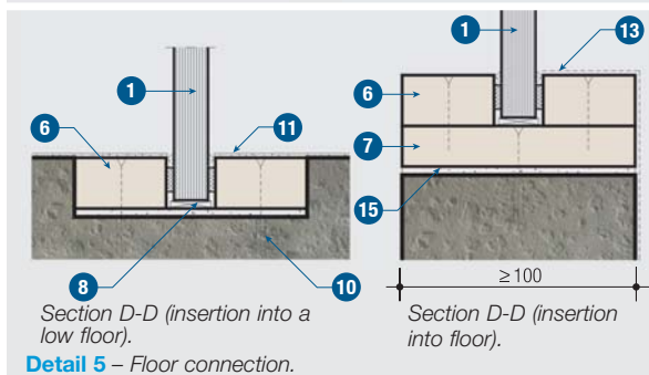
Detail 5 – Floor connection.
