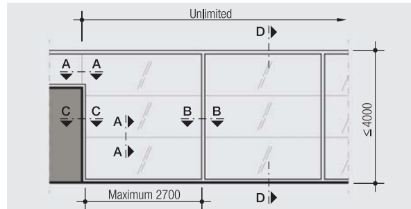
Detail 1 – Elevation (Horizontal unframed joints).
