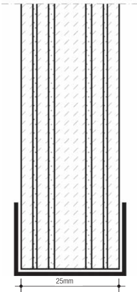
Type 1 – Standard glass.
