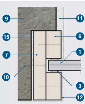
Detail 3 – (a) Wall connection (Section C-C).
