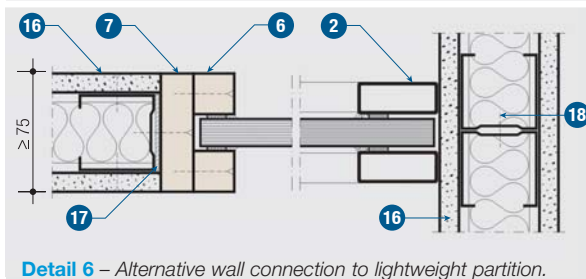
Detail 6 – Alternative wall connection to lightweight partition.
