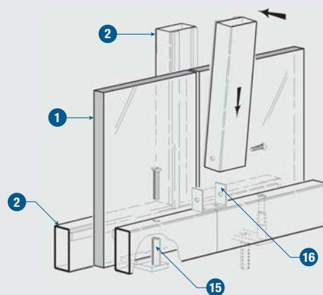
Detail 8 – Screw fixed frames assembly.
