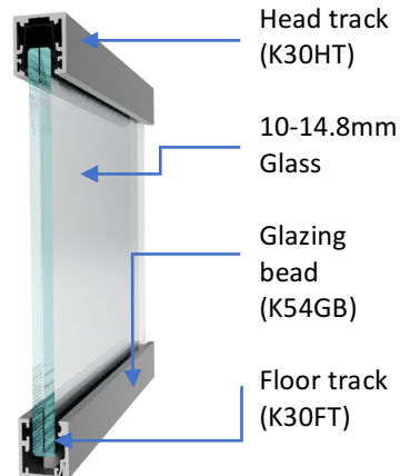
Standard Single Glazed Head and Base Detail
