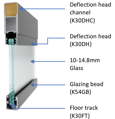
Standard +/-25mm Deflection Head and Base Detail
