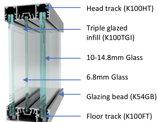
Triple Glazed Head and Base Detail
