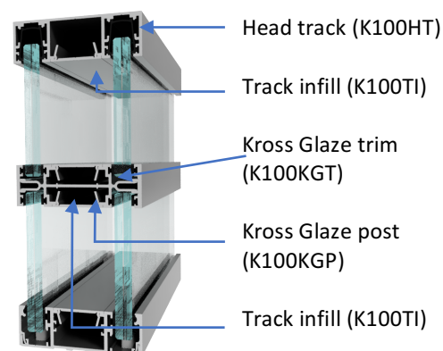
Double Glazed with Kross Glaze Transom
