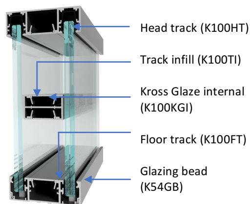
Double Glazed with Kross Glaze Internal
