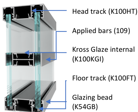
Double Glazed with Applied Kross Glaze
