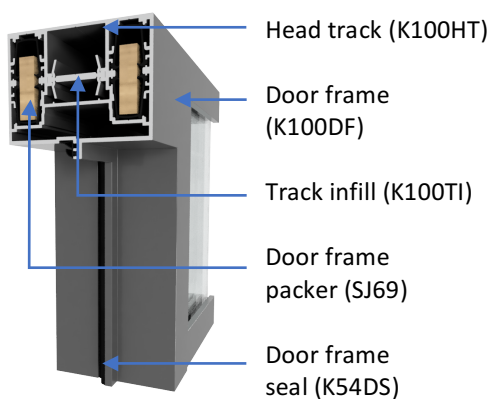
Standard Full Height Door Frame Detail
