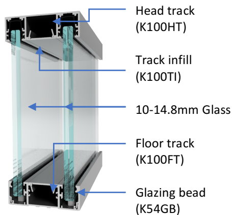
Standard Double Glazed Head and Base Detail
