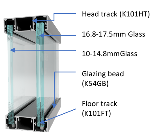
Standard Double Glazed Head and Base Detail
