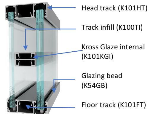
Double Glazed with Kross Glaze Internal
