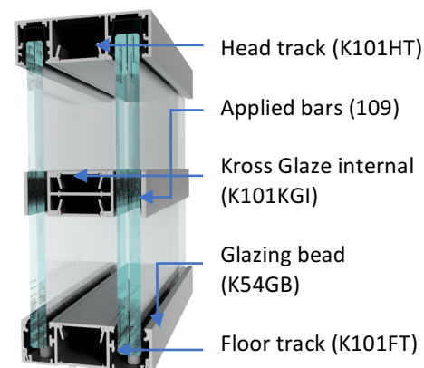
Double Glazed with Applied Kross Glaze
