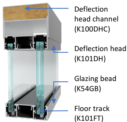
Standard +/-25mm Deflection Head and Base Detail Detail
