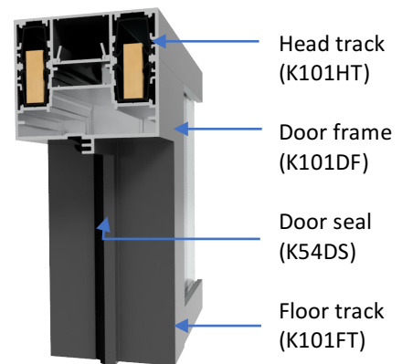
Standard Triple Glazed Head and Base Detail
