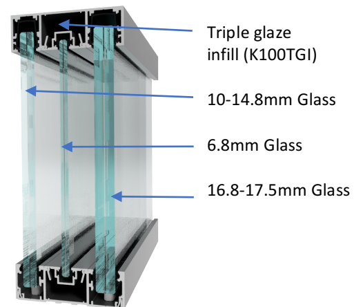
Standard Triple Glazed Head and Base Detail
