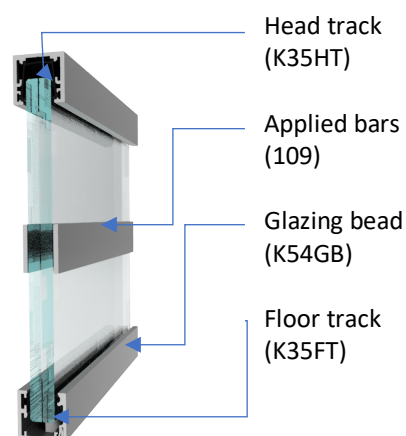
Single Glazed with Applied Kross Glaze Bars
