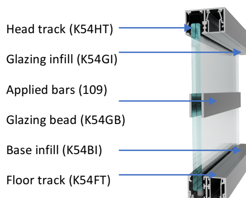
Offset Single Glazed Kross Glaze Applied Bars Detail
