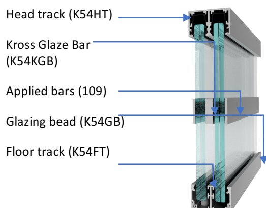
Double Glazed Kross Glaze Applied Bars Detail
