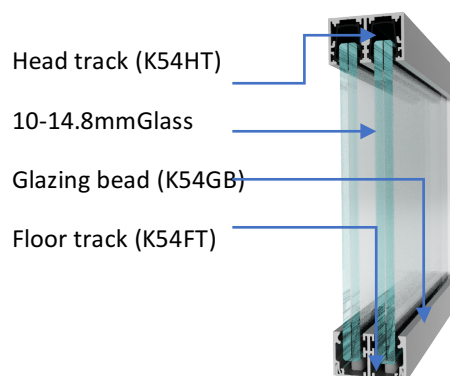
Standard Double Glazed Head and Base Detail
