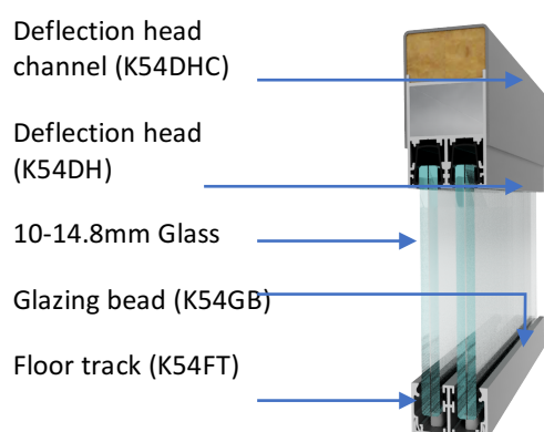
Standard +/-25mm Deflection Head and Base Detail
